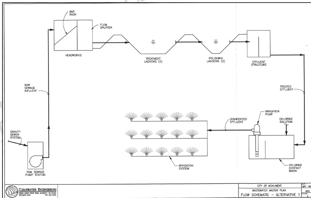
Figure 2-2: City of Monument Flow Schematic
