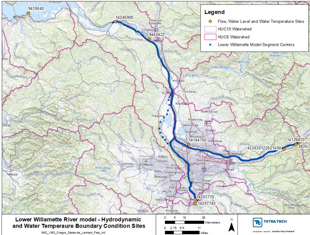
Figure 3-2. Monitoring stations for deriving boundary conditions in the Lower Willamette River Model
