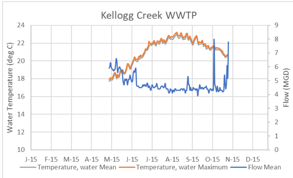
Figure 3-40. Kellogg Creek WWTP 2015 flow and water temperature.
