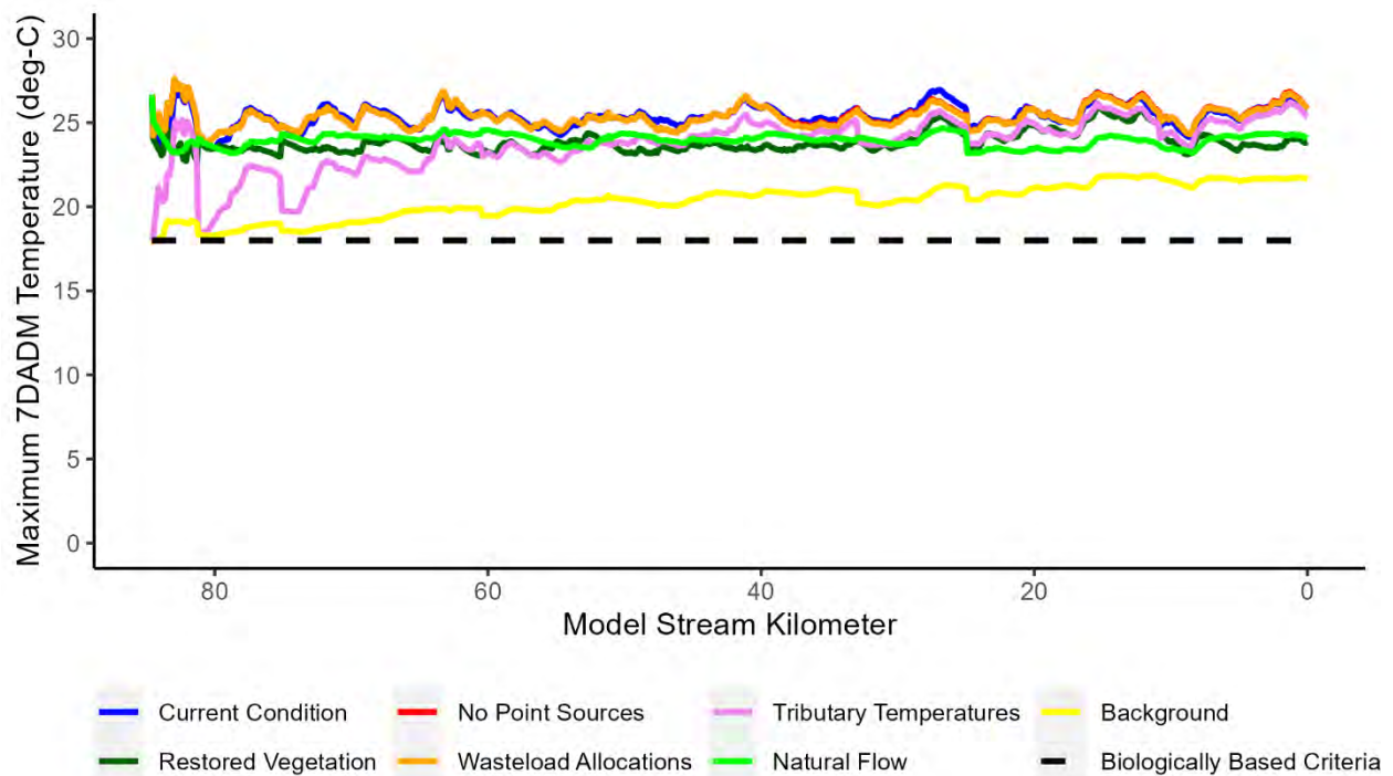
Figure 4-19: Maximum 7-Day Average Daily Maximum stream temperature for all model scenarios for the Pudding River.
