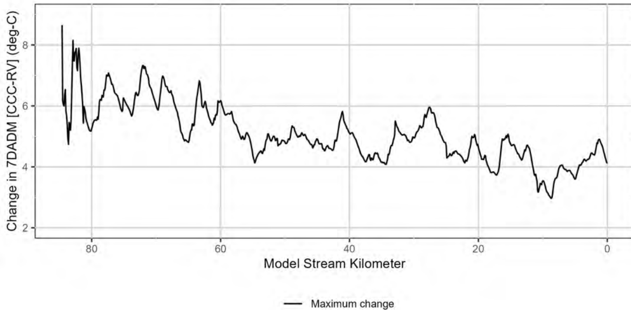
Figure 4-47: Change in maximum 7-Day Average Daily Maximum stream temperatures between the Background and Current Condition scenarios for the Pudding River over the entire model period.
