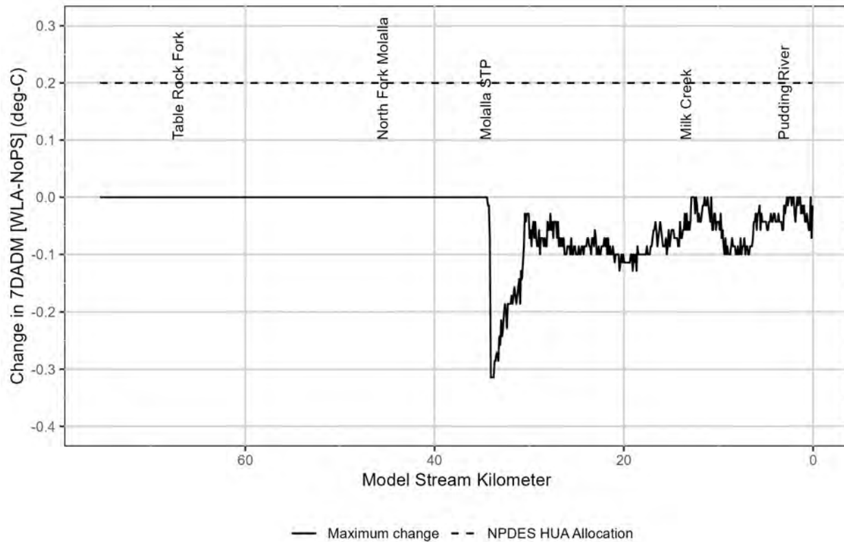
Figure 4-16: Change in maximum 7-Day Average Daily Maximum stream temperatures between the Wasteload Allocations and No Point Sources scenarios for the Molalla River over the entire model period.
