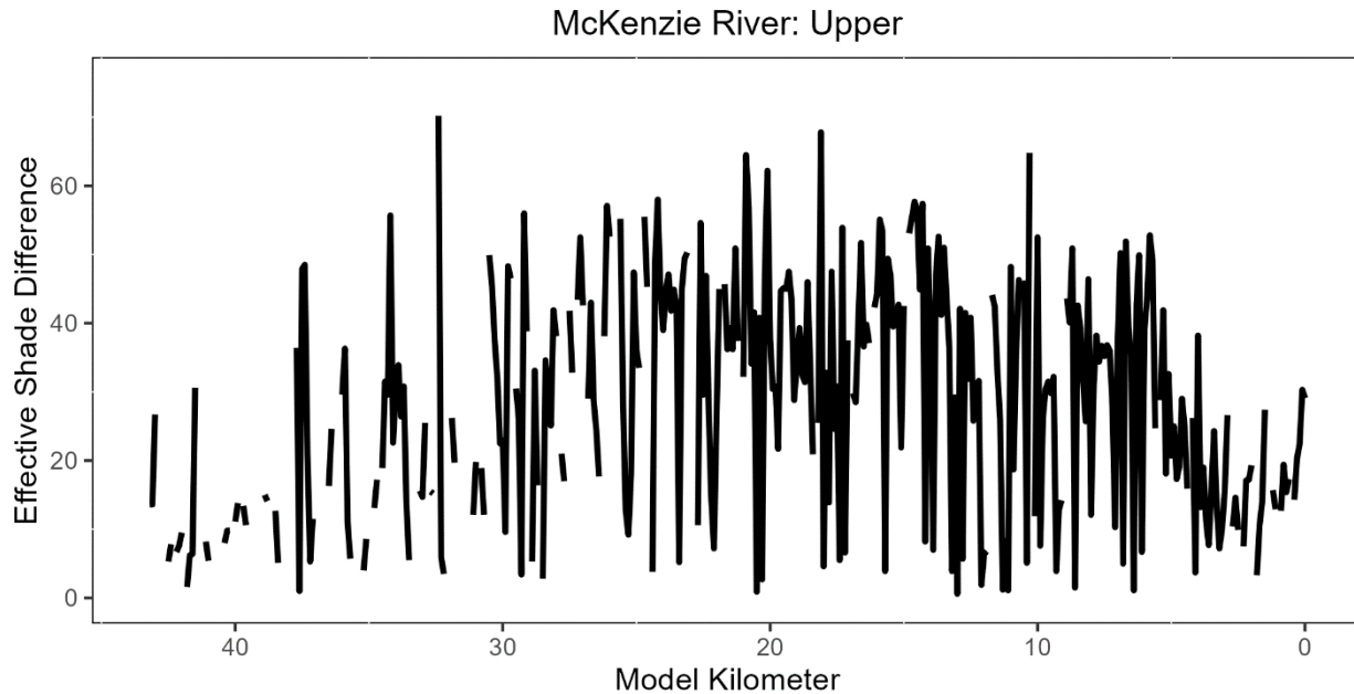
Figure 4-74: Percentage point difference between effective shade from the Current Condition and Restored Vegetation scenarios on 9/3/1999 for the upper McKenzie River. Missing values indicate that the shade difference is negative due to instances of higher effective shade in the Current Condition scenario versus the Restored Vegetation scenario.
