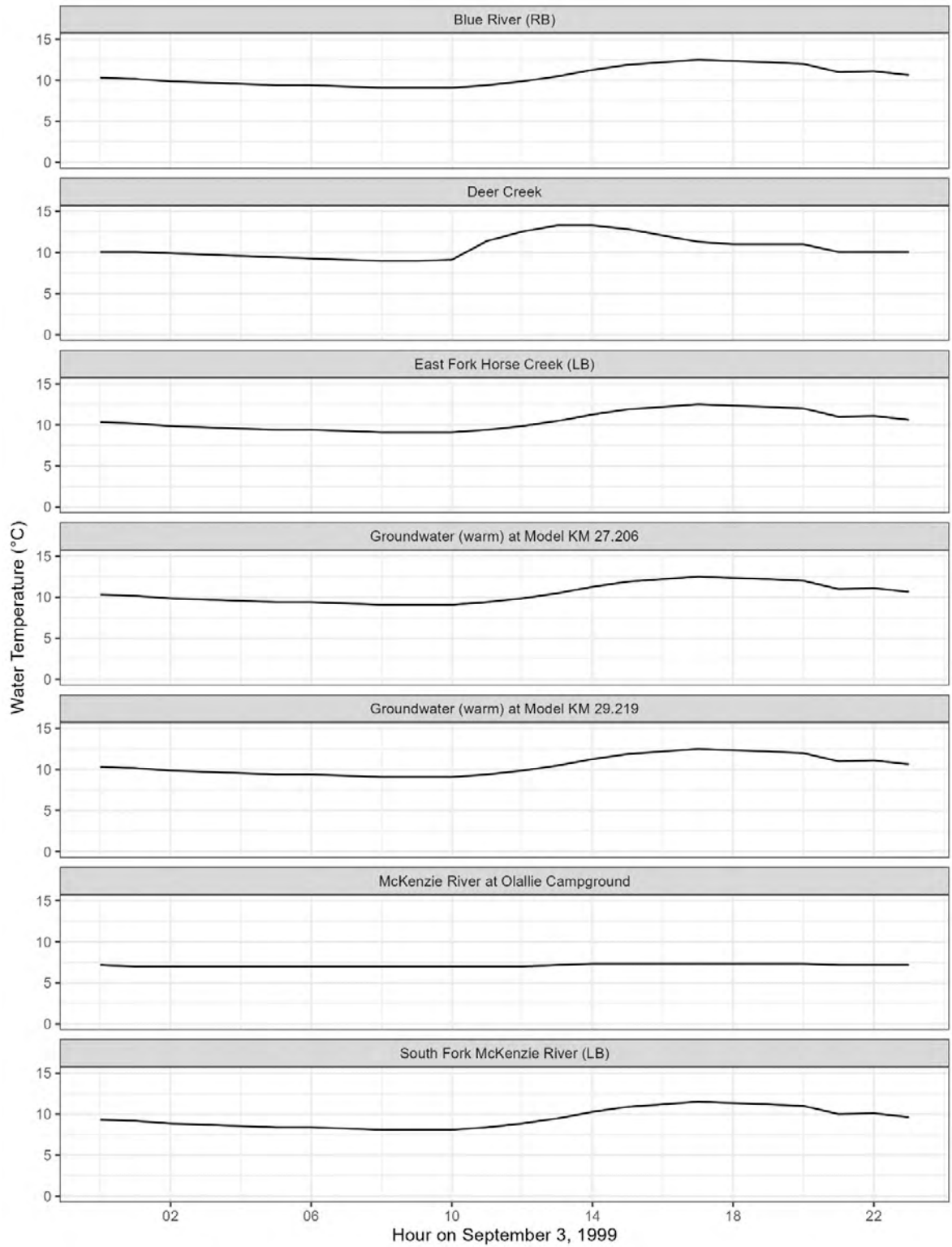
Figure 3-200: Boundary condition, ground water and tributary water temperature inputs to the upper McKenzie River model.
