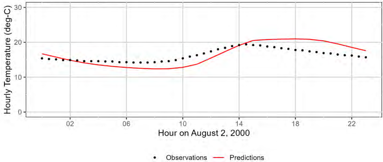
23742-ORDEQ: Crabtree Creek at Main Line Bridge Model Kilometer 50.7
