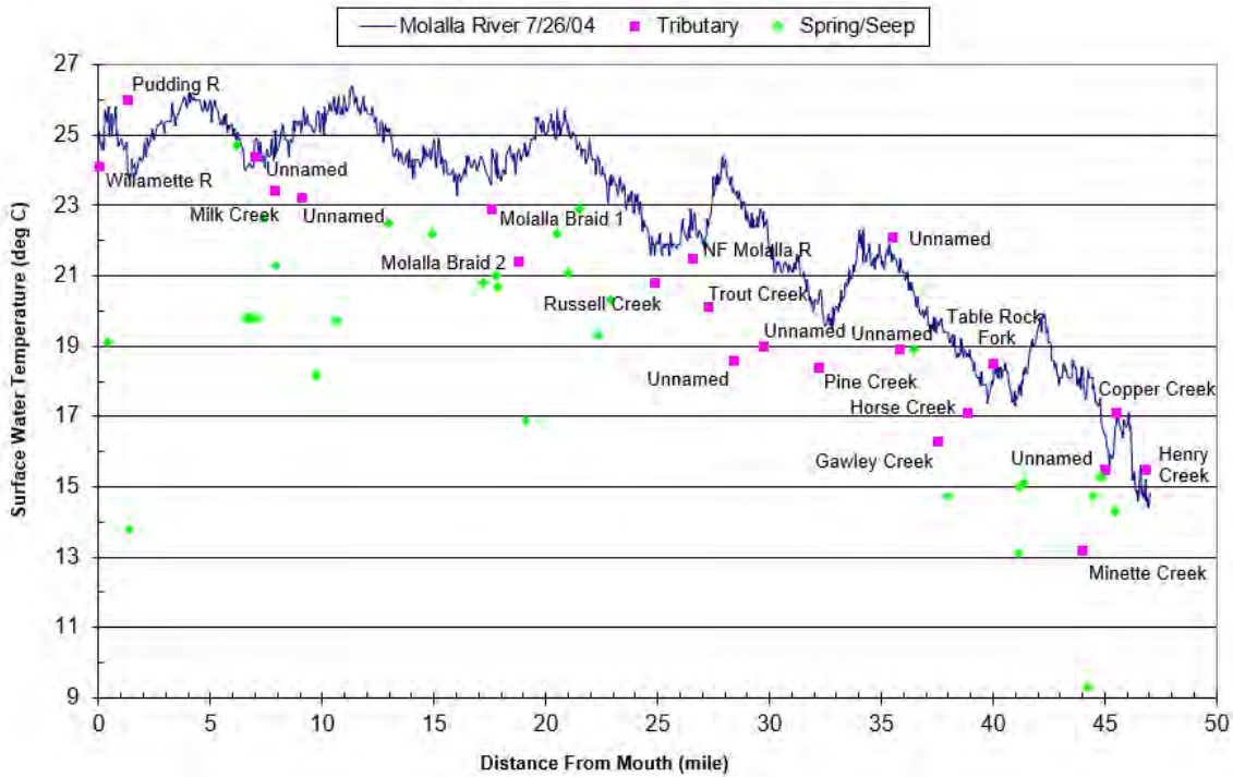
Figure 2-5: TIR temperatures for the Molalla River in the Molalla-Pudding Subbasin.
