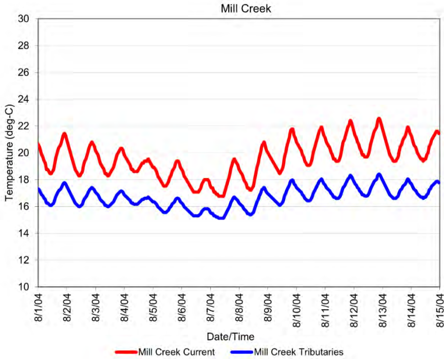
Figure 4-41: Current temperatures for Mill Creek and theoretical tributary temperatures that meet the 18 deg-C biological criterion.
