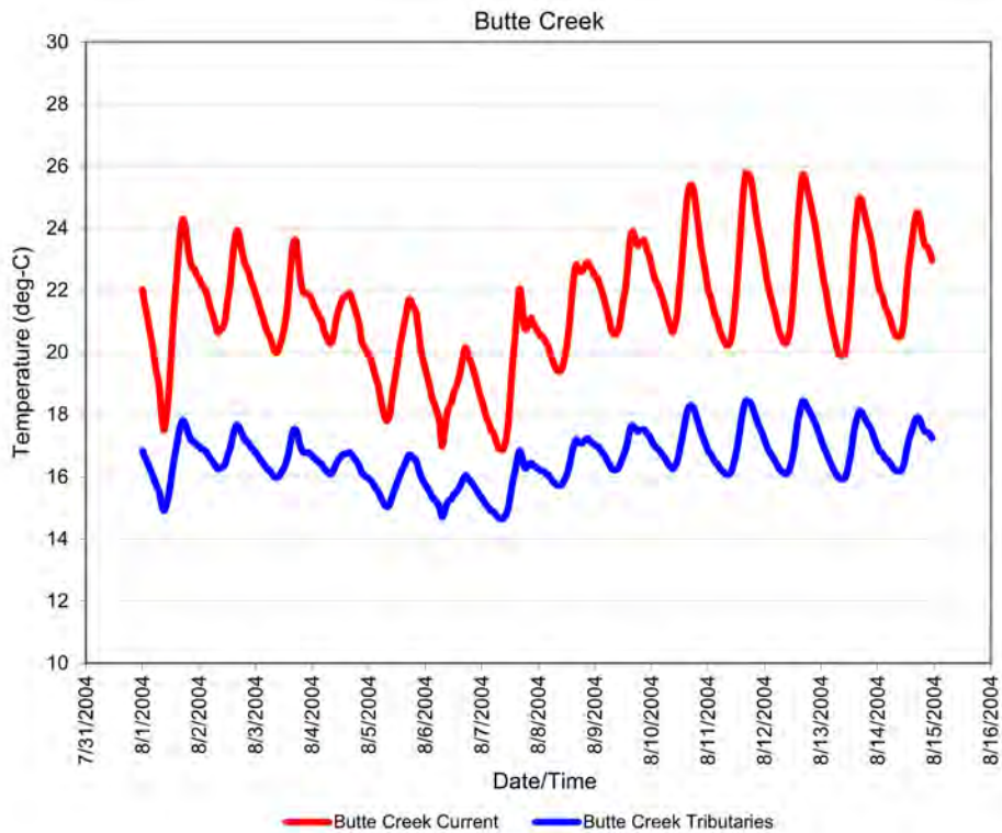
Figure 4-45: Current temperatures for Butte Creek and theoretical tributary temperatures that meet the 18 deg-C biological criterion.
