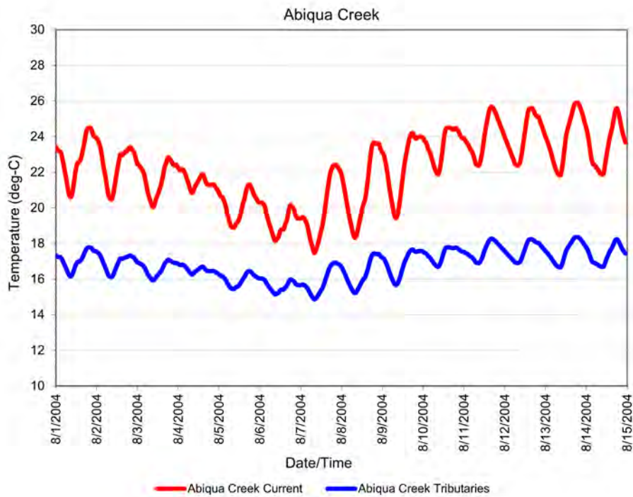
Figure 4-39: Current temperatures for Abiqua Creek and theoretical tributary temperatures that meet the 18 deg-C biological criterion.
