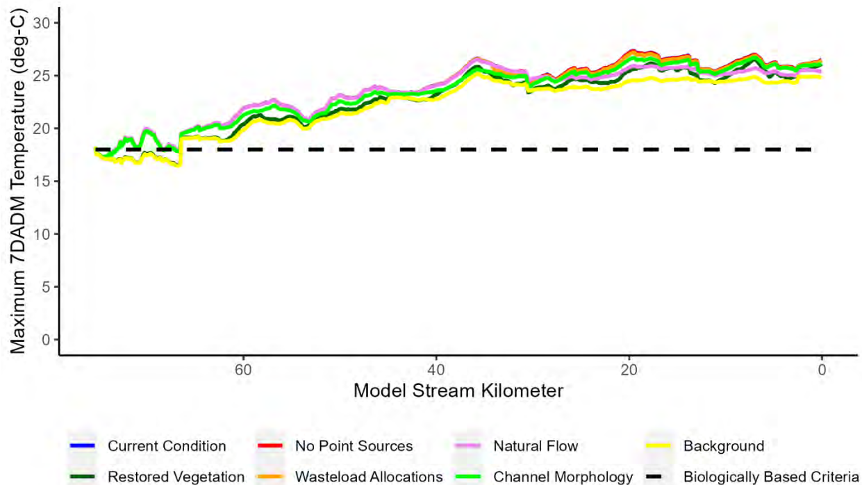
Figure 4-9: Maximum 7-Day Average Daily Maximum stream temperature for all model scenarios for the Molalla River.
