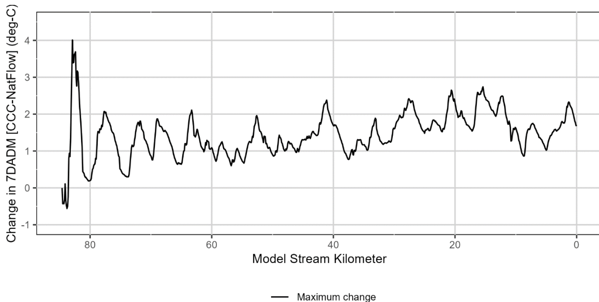
Figure 4-31: Change in maximum 7-Day Average Daily Maximum stream temperatures between the Current Condition and Natural Flow scenarios for the Pudding River over the entire model period.
