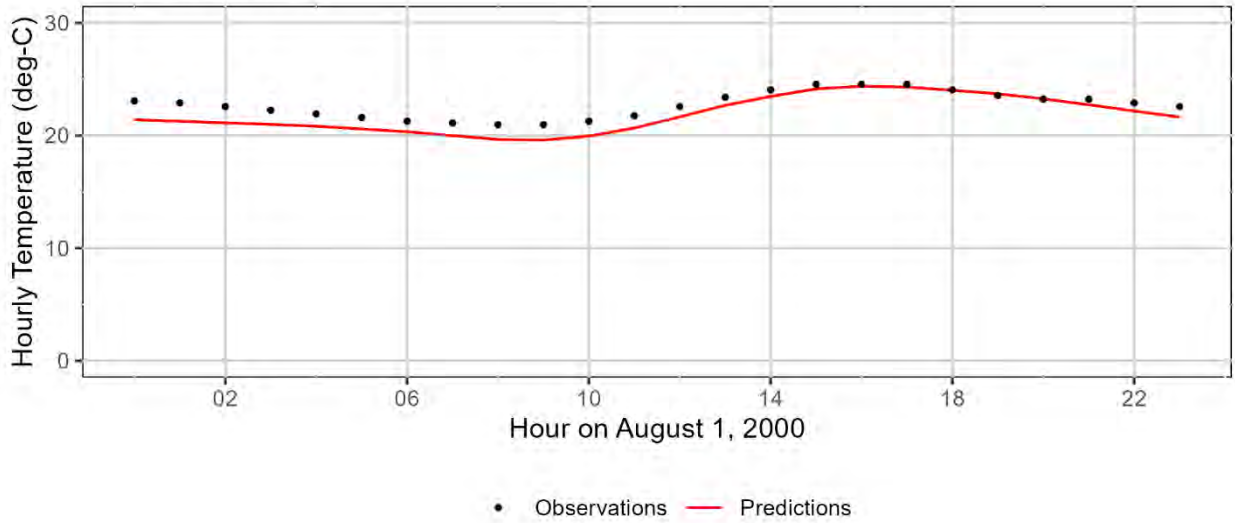
BLMNF: North Fork County Park Model Kilometer 4.4
