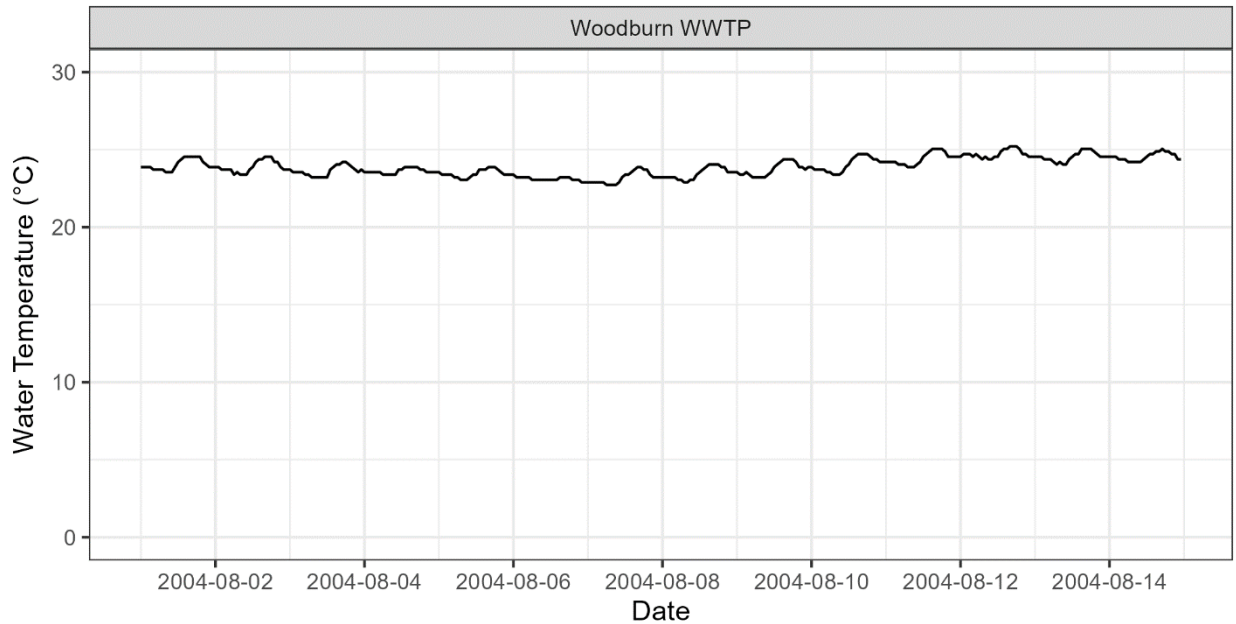
Figure 3-68: Pudding River current condition calibration model setup up for Woodburn WWTP effluent temperatures.
