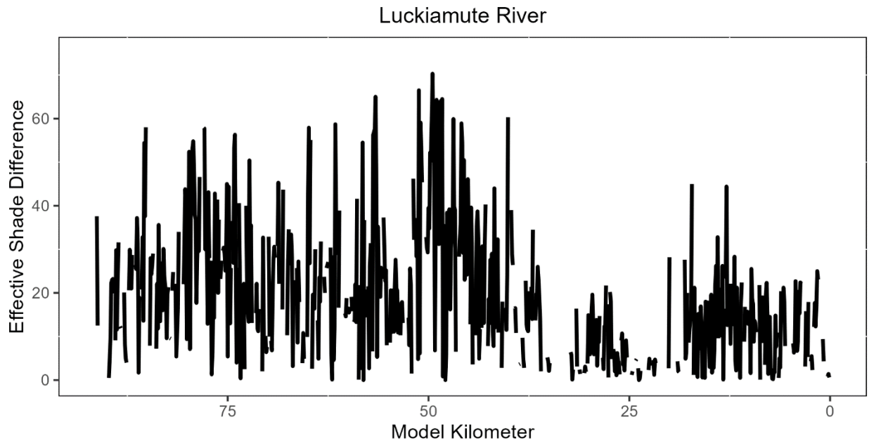
Figure 4-66: Percentage point difference between effective shade from the Current Condition and Restored Vegetation scenarios on 8/12/2001 for the Luckiamute River. Missing values indicate that the shade difference is negative due to instances of higher effective shade in the Current Condition scenario versus the Restored Vegetation scenario.
