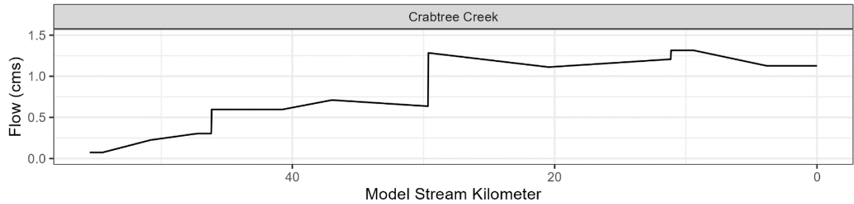
Figure 3-140: Boundary condition and mainstem flow inputs to the Crabtree Creek model.
