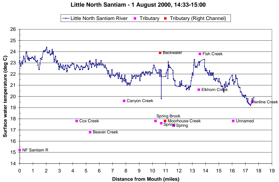
Figure 2-7: TIR temperatures for the Little North Santiam River in the North Santiam Subbasin.
