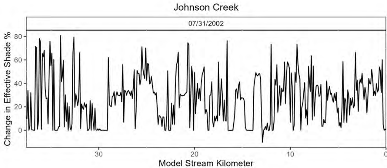
Figure 4-3: Comparison of effective shade from the Current Condition and Restored Vegetation scenarios for Johnson Creek.
