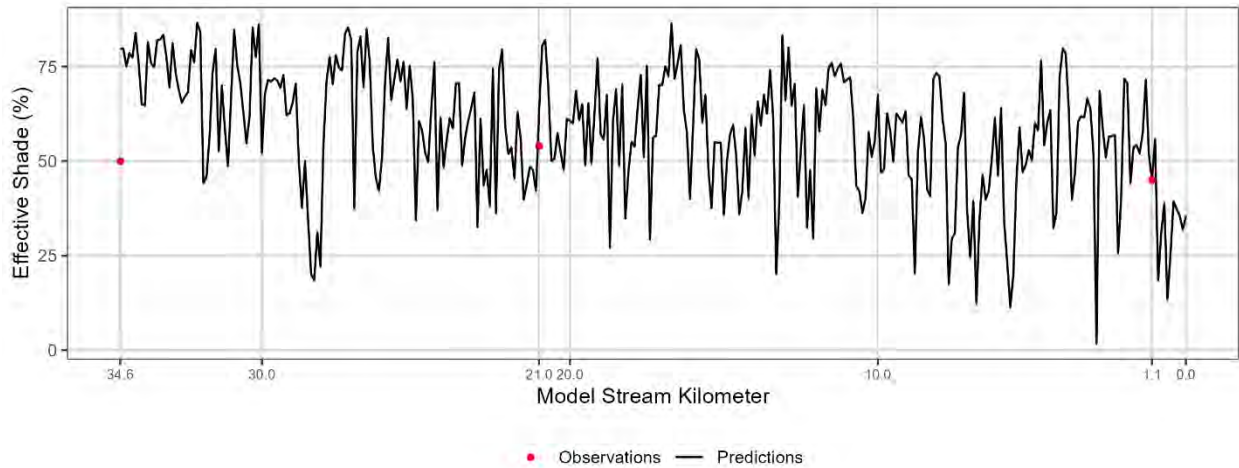
Figure 3-242: Mosby Creek field observed and model-predicted effective shade.
