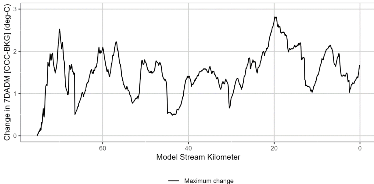
Figure 4-18: Change in maximum 7-Day Average Daily Maximum stream temperatures between the Background and Current Condition scenarios for the Molalla River over the entire model period.
