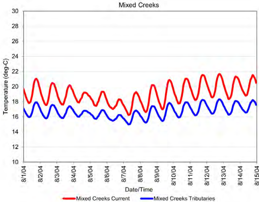
Figure 4-46: Current temperatures for mixed creeks (Mill Creek, Zollner Creek, Upper Pudding River, and groundwater) and theoretical tributary temperatures that meet the 18 deg-C biological criterion.
