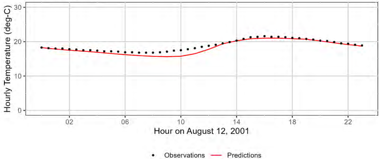
Figure 3-171: Luckiamute River measured and model-predicted hourly temperatures at monitoring station 25486-ORDEQ.
