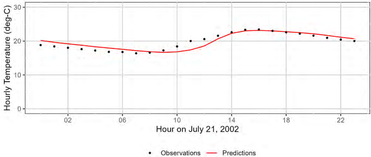
28101-ORDEQ: Mosby Creek Above Cedar Creek Model Kilometer 21
