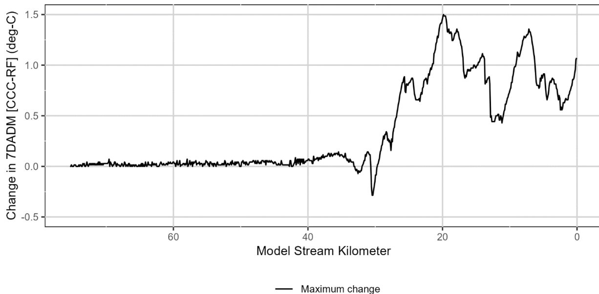
Figure 4-17: Change in maximum 7-Day Average Daily Maximum stream temperatures between the Restored Flow and Current Condition scenarios for the Molalla River over the entire model period.
