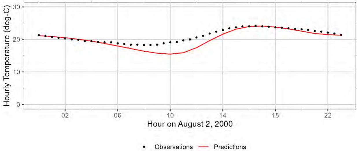
23768-ORDEQ: Crabtree Creek ar Larwood Bridge Model Kilometer 29.7
