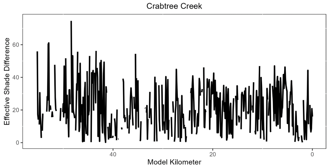
Figure 4-61: Comparison of effective shade from the Current Condition and Restored Vegetation scenarios for Crabtree Creek.
