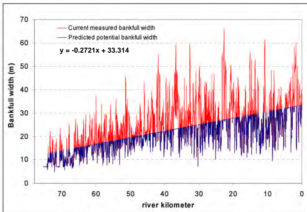
Figure 4-10: GIS measured bankfull width compared with predicted bankfull width. A regression was performed of the moving median of bankfull width from headwaters to mouth. Modified
