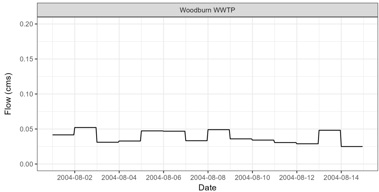
Figure 4-22: Pudding River current condition scenario model setup for Woodburn WWTP effluent flow rates.
