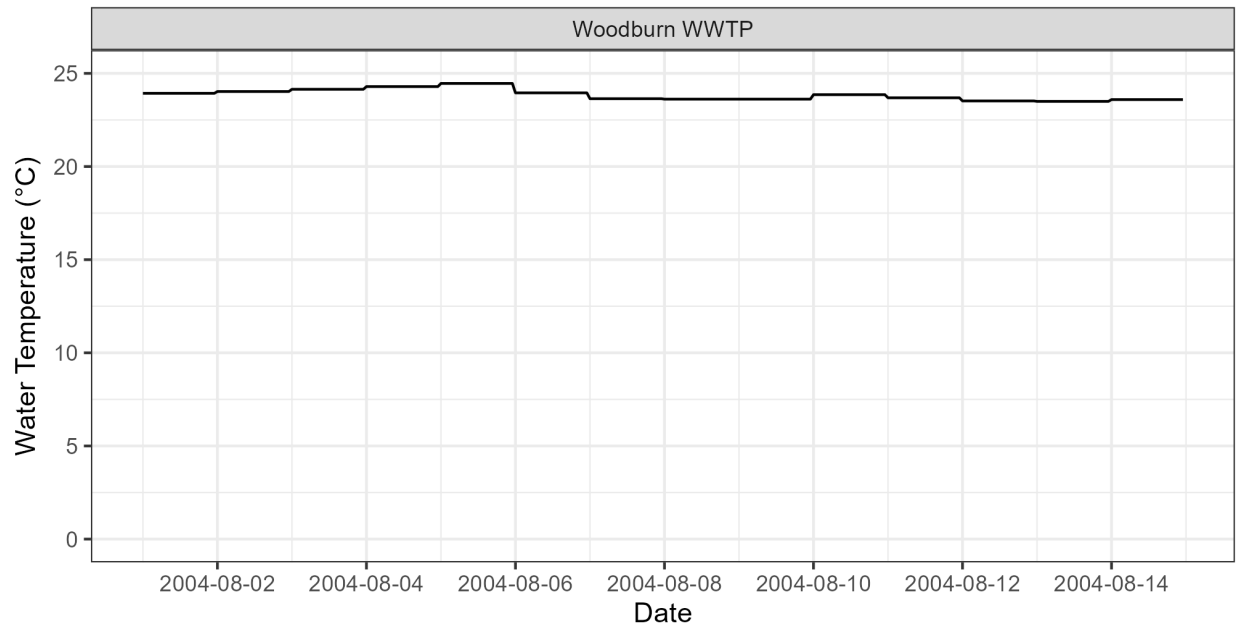
Figure 4-21: Pudding River current condition scenario model setup for Woodburn WWTP effluent temperatures.
