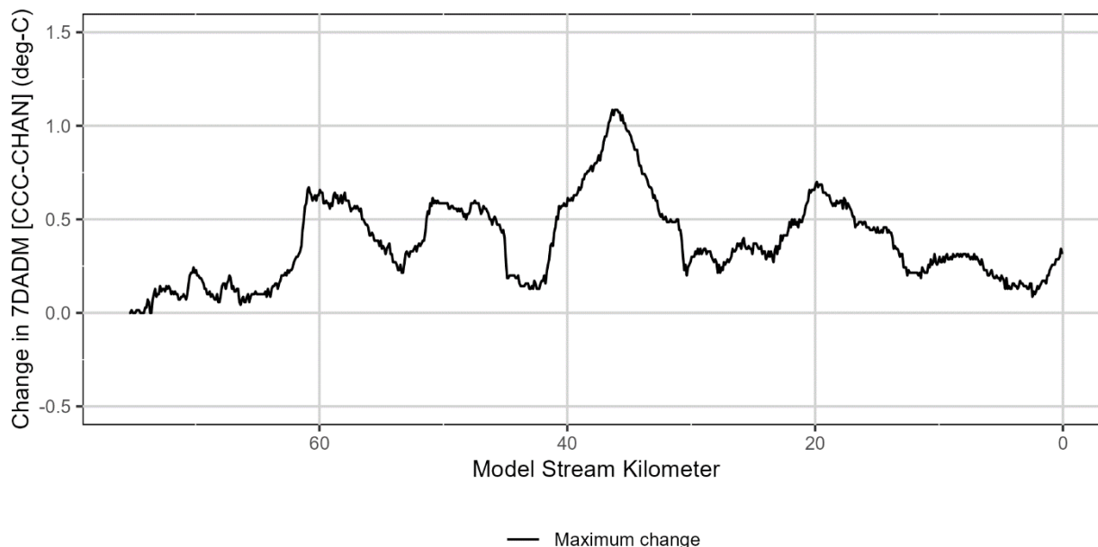
Figure 4-15: Change in maximum 7-Day Average Daily Maximum stream temperatures between the Channel Morphology and Current Condition scenarios for the Molalla River over the entire model period.
