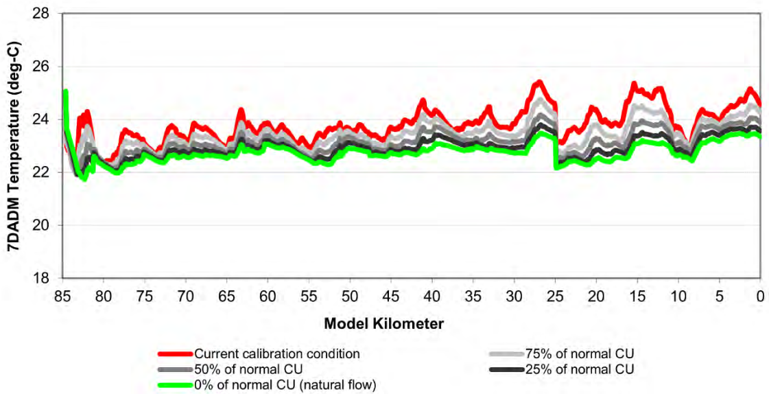
Figure 4-36: Maximum 7-Day Average Daily Maximum stream temperature for all consumptive use model scenarios for the Pudding River.
