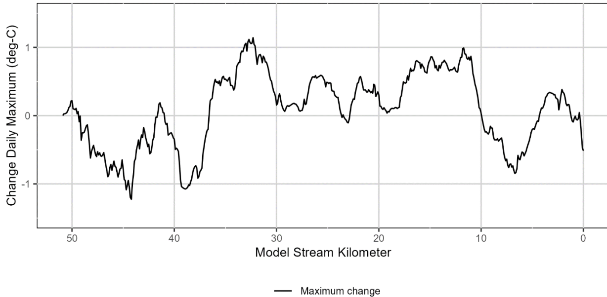
Figure 4-53: Change in the daily maximum stream temperatures between the Current Condition and Restored Vegetation model scenarios for Thomas Creek over the entire model period.
