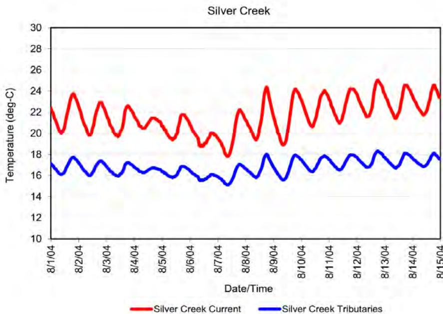
Figure 4-38: Current temperatures for Silver Creek and theoretical tributary temperatures that meet the 18 deg-C biological criterion.
