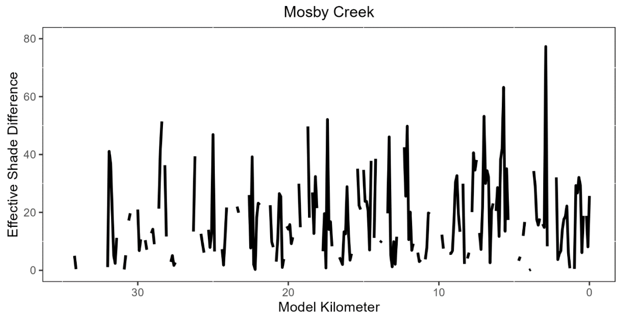
Figure 4-82: Comparison of effective shade from the Current Condition and Restored Vegetation scenarios for Mosby Creek.
