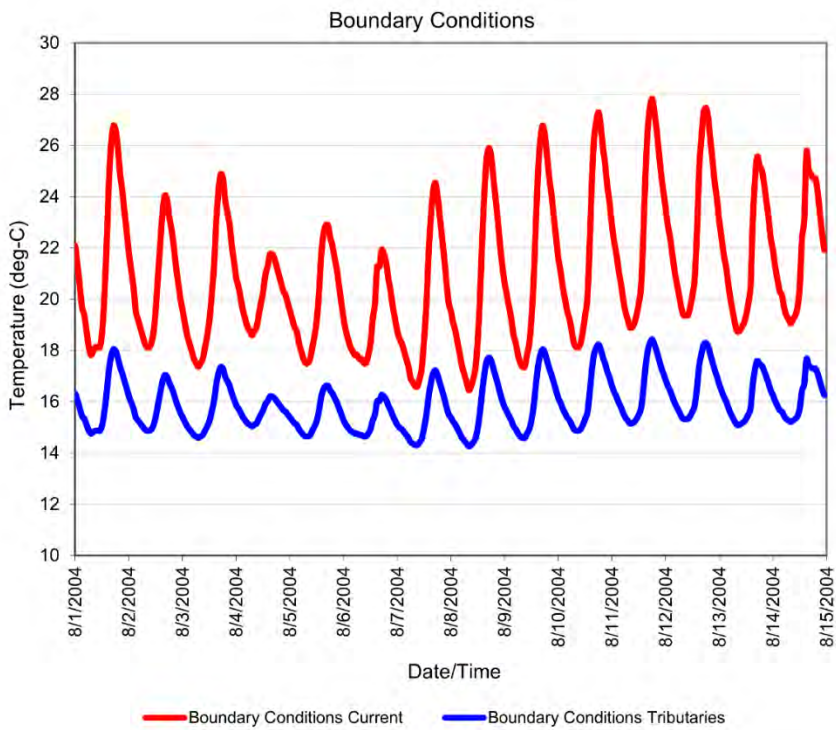
Figure 4-41: Current temperatures for Mill Creek and theoretical tributary temperatures that meet the 18 deg-C biological criterion.
