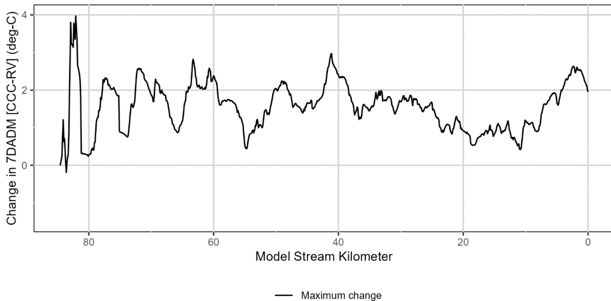
Figure 4-23: Change in the maximum 7-Day Average Daily Maximum stream temperatures between Current Condition and Restored Vegetation scenarios for the Pudding River over the entire model period.
