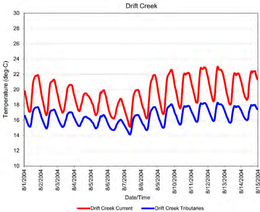
Figure 4-43: Current temperatures for Drift Creek and theoretical tributary temperatures that meet the 18 deg-C biological criterion.
