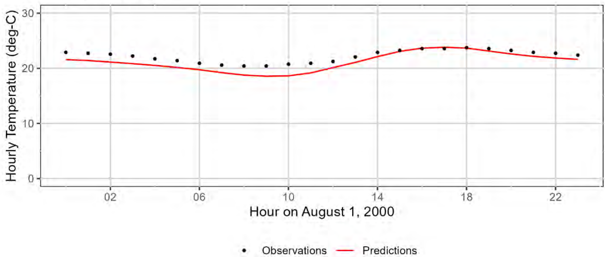
S88442: Model Node 4 Model Kilometer 7.6
