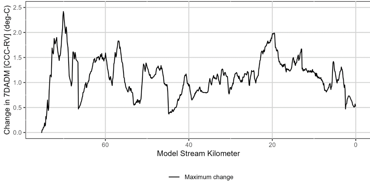
Figure 4-12: Change in the maximum 7-Day Average Daily Maximum stream temperatures between Current Condition and Restored Vegetation scenarios for the Molalla River over the entire model period.
