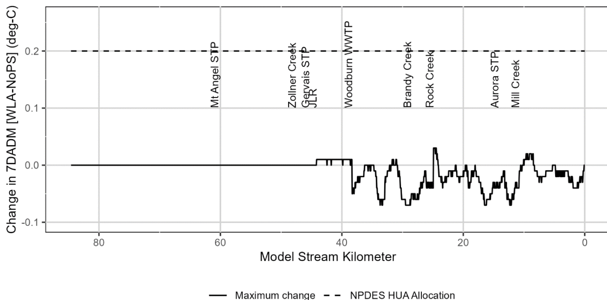
Figure 4-30: Change in maximum 7-Day Average Daily Maximum stream temperatures between the Wasteload Allocations and No Point Sources scenarios for the Pudding River over the entire model period.
