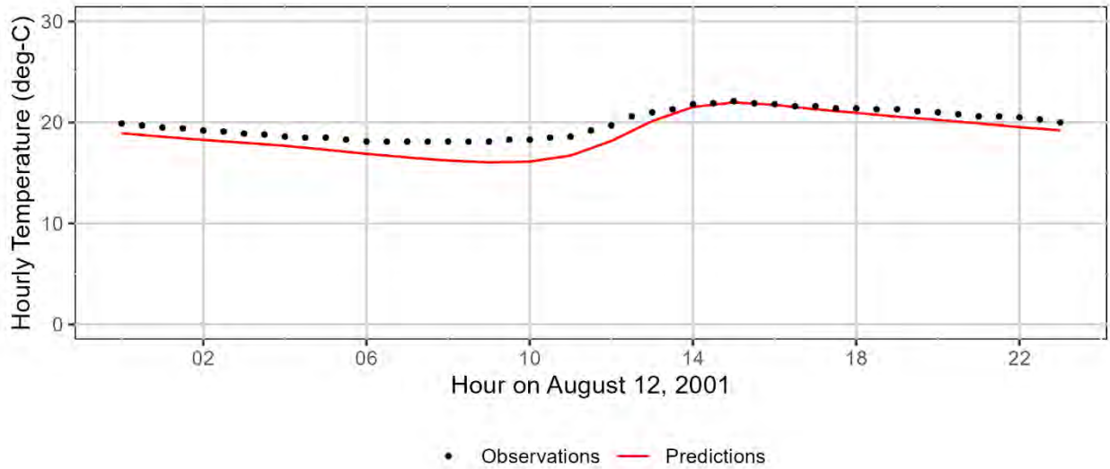
Figure 3-170: Luckiamute River measured and model-predicted hourly temperatures at monitoring station 11111-ORDEQ.
