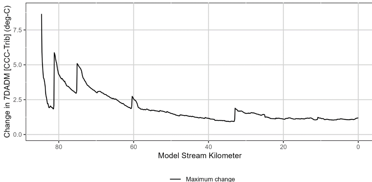
Figure 4-37: Change in maximum 7-Day Average Daily Maximum stream temperatures between the Current Condition and Tributary Temperatures scenarios for the Pudding River over the entire model period.
