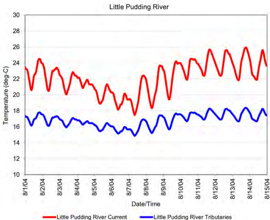
Figure 4-40: Current temperatures for the Little Pudding River and theoretical tributary temperatures that meet the 18 deg-C biological criterion.
