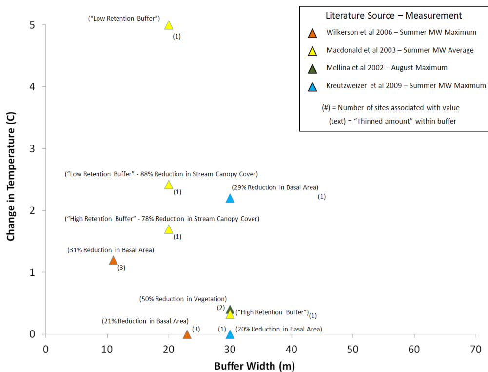
Figure 1-5: Observed temperature response associated with “thinned” riparian buffers with adjacent clearcut harvest. Corresponding references and measurement methods and types are listed in the legend. Abbreviation: MW = mean weekly (Source – Leinenbach et al 2013).
