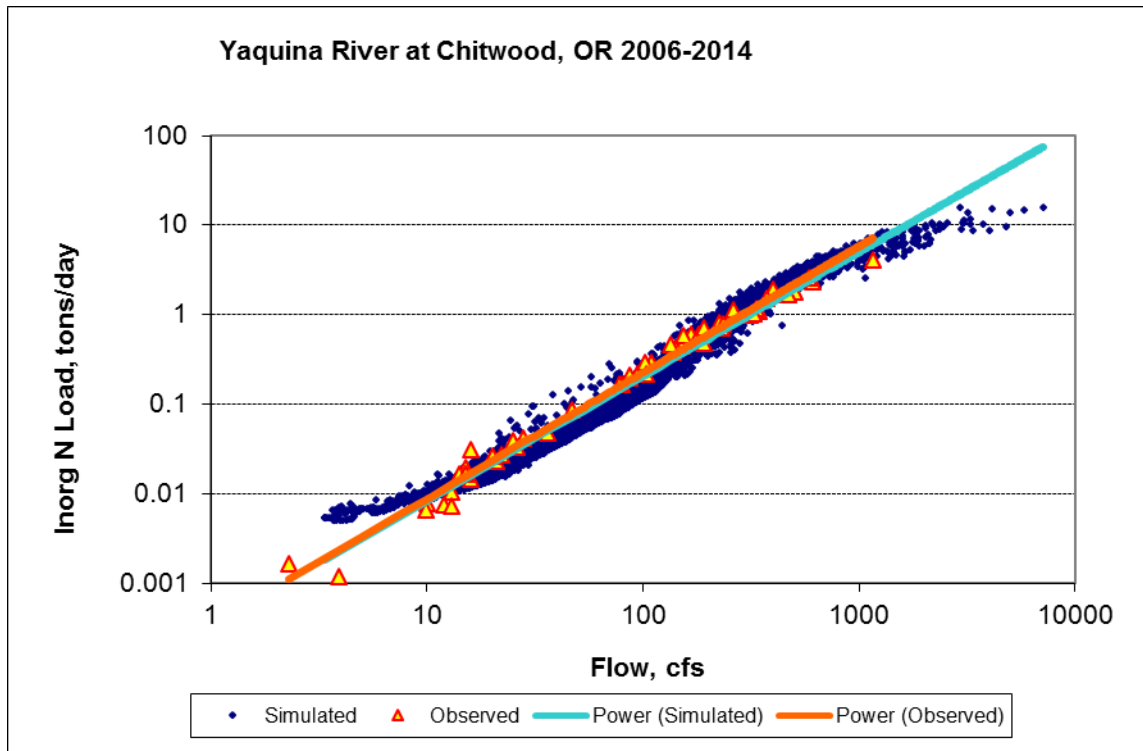
Figure 34. Inorganic N Load versus Flow, Validation Period
