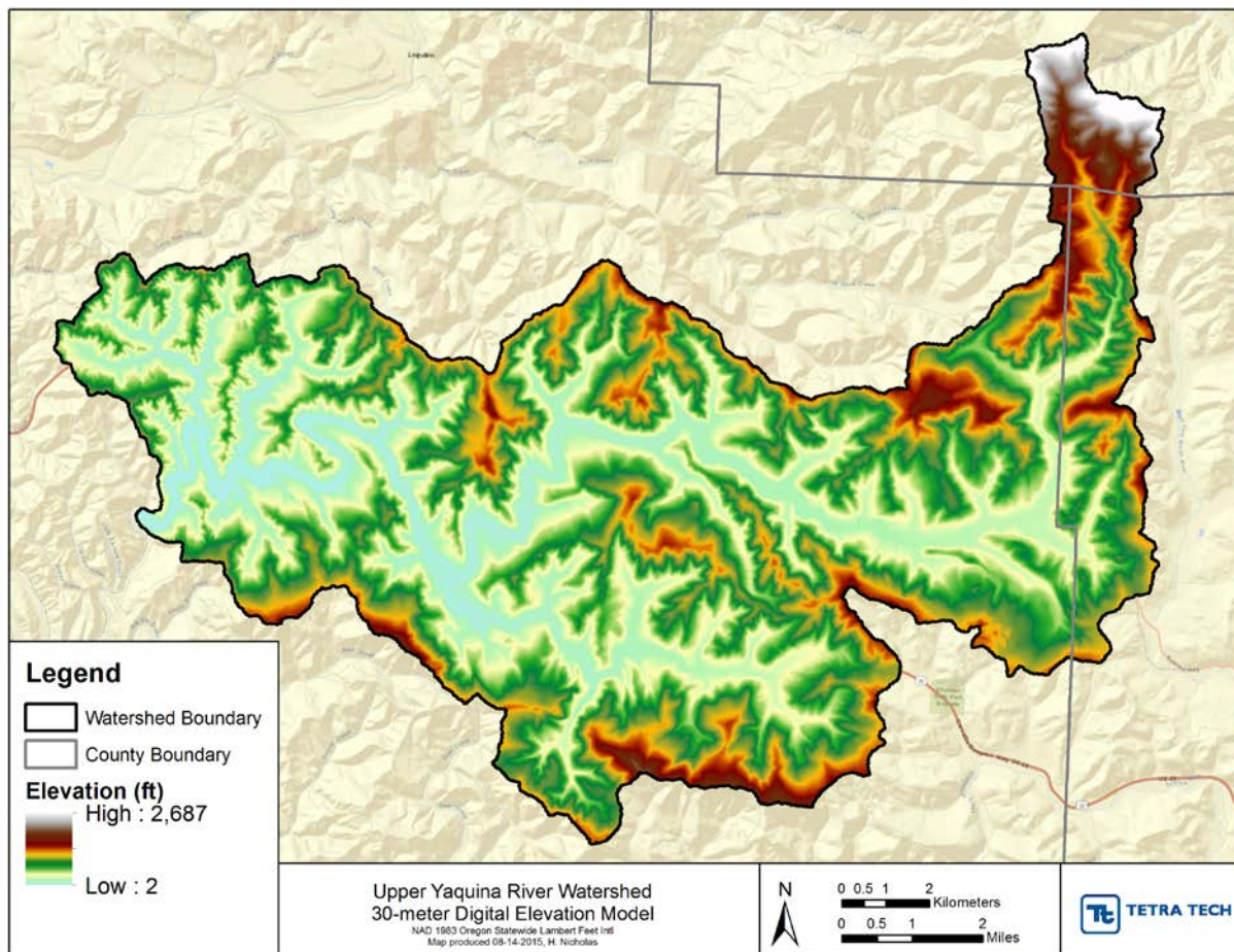
Figure 2. Elevation in the Upper Yaquina River watershed.
