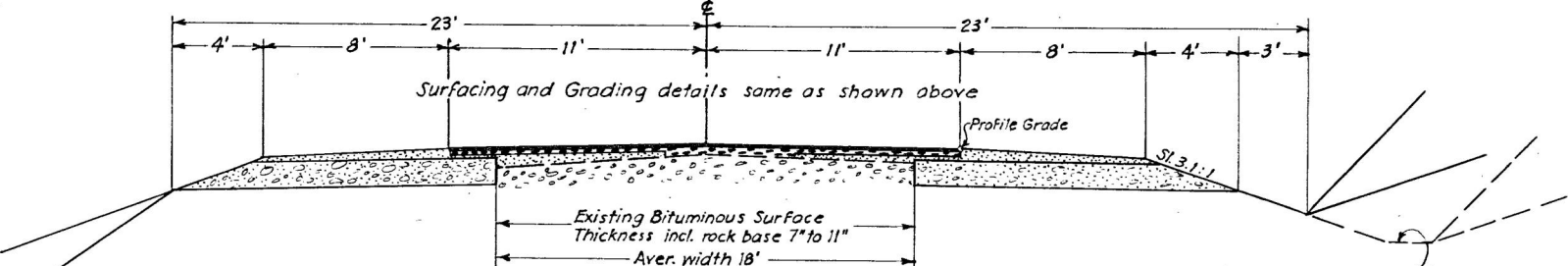
Resurfacing Section Sta. 462 to Sta. 514 excepting new work.
