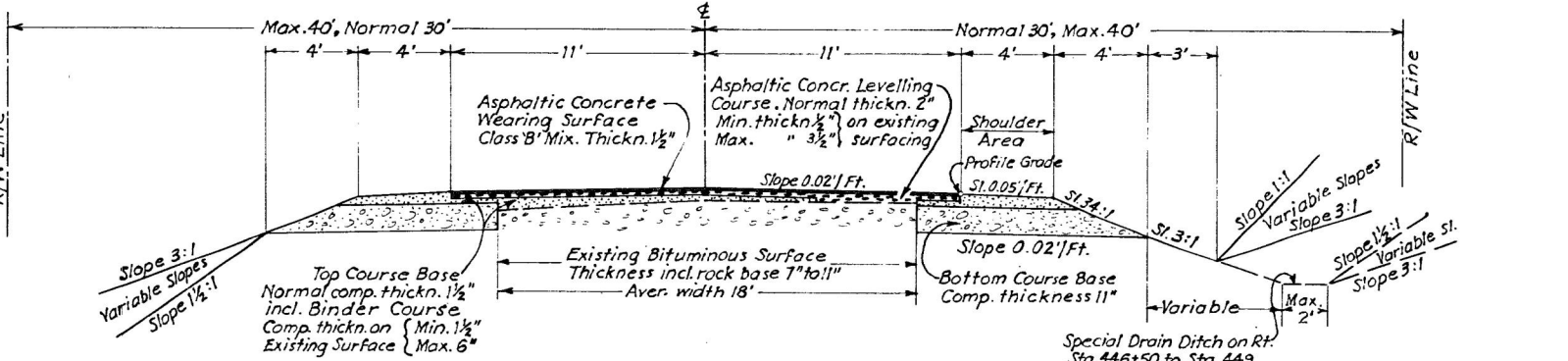
Resurfacing Section Sta. 416+75 to Sta. 462 excepting new work.
