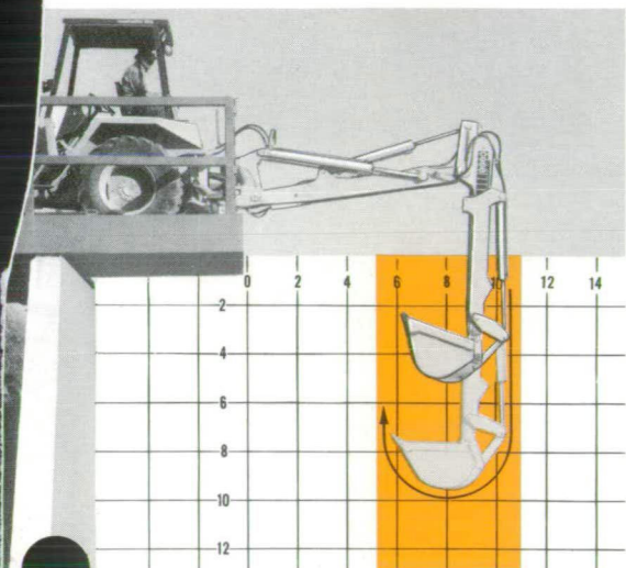
Hydraulic telescoping dipper permits digging of vertical holes.
