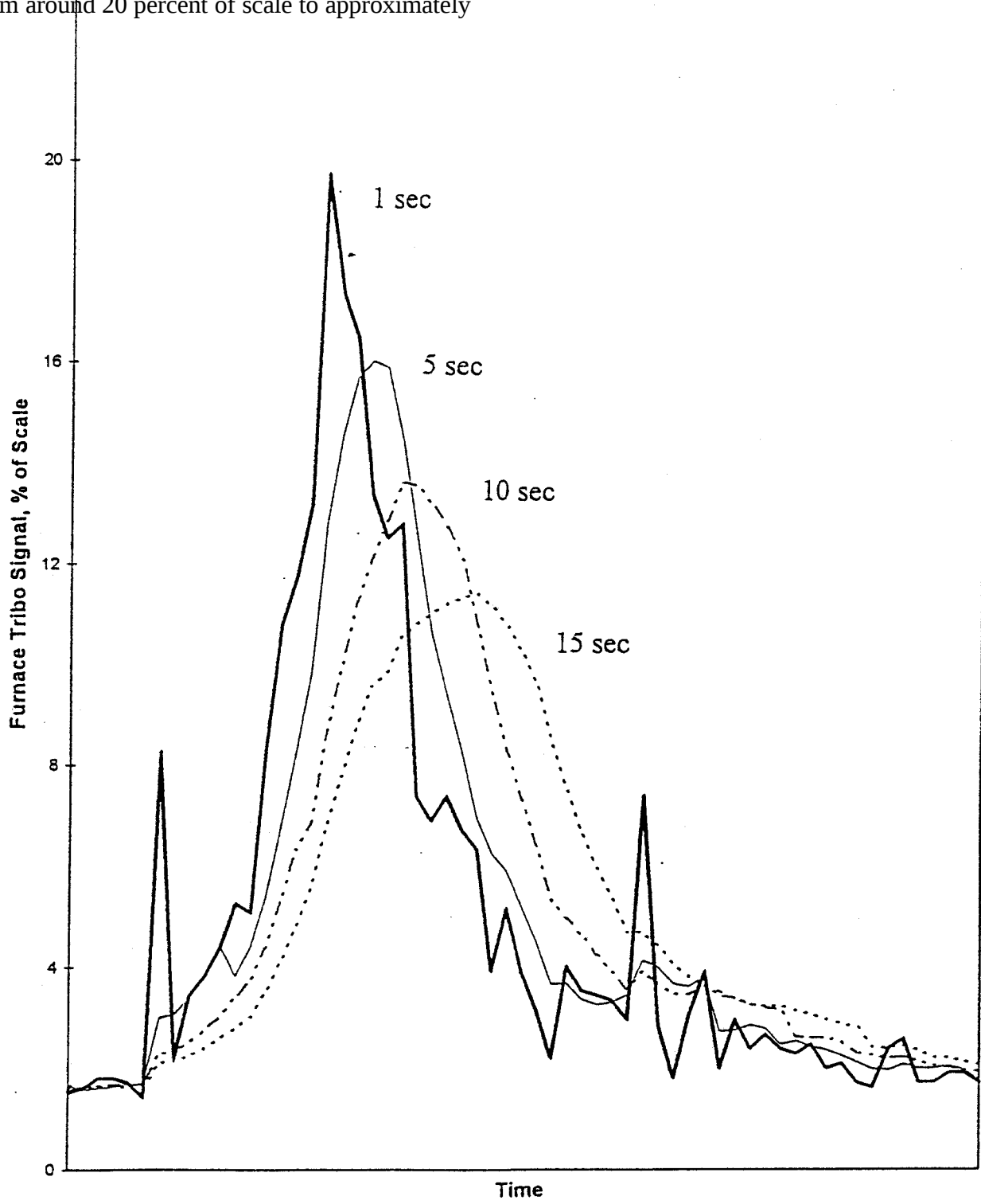
Figure 7. Effect of response time on a typical baghouse cleaning peak.
