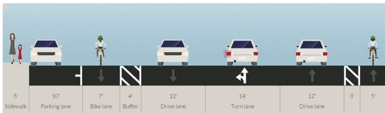
Exhibit 5-4. Example Cross-section Looking North on W 6 th Street Between Snipes Street and Hostetler Street (Source: www.streetmix.net )
