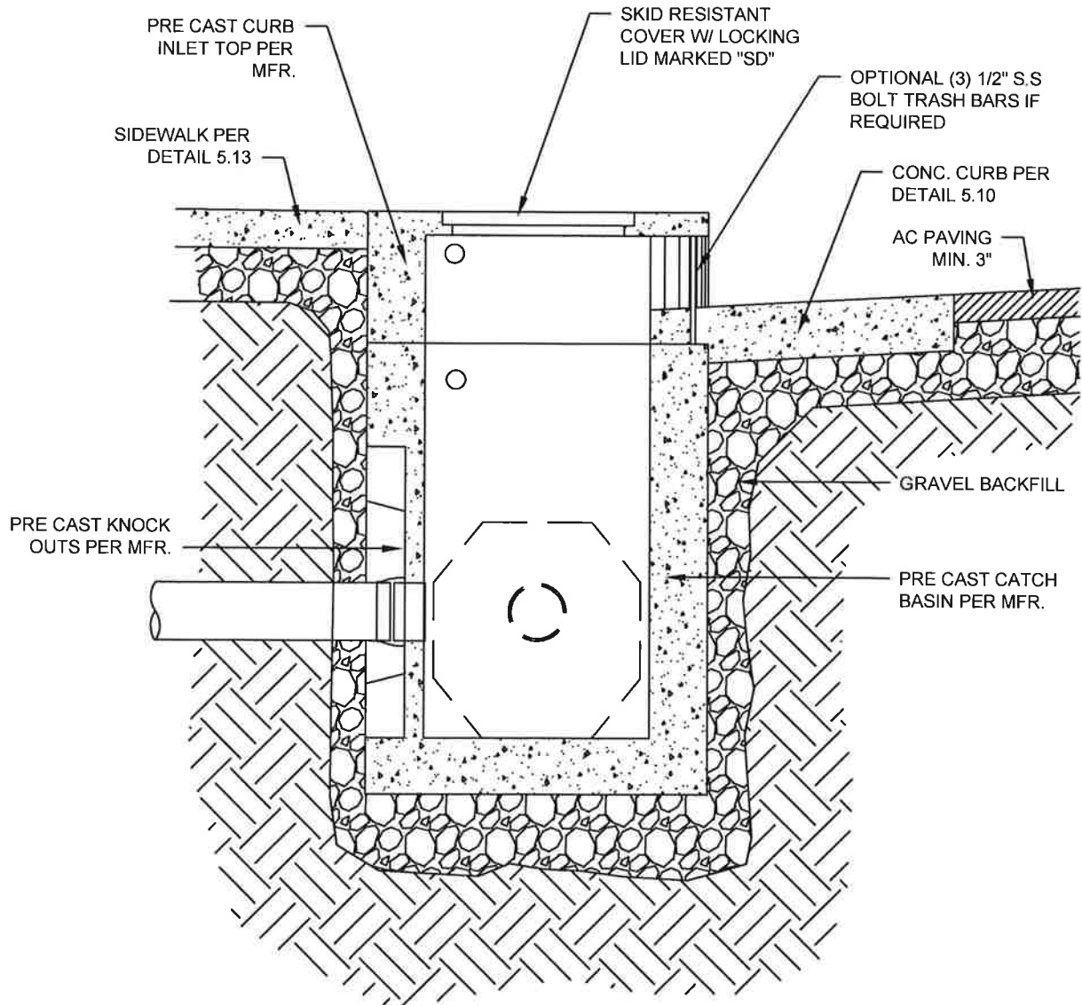
SECTION
