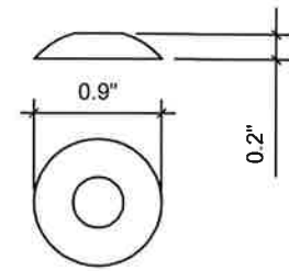
TRUNCATED DOME DETAIL
