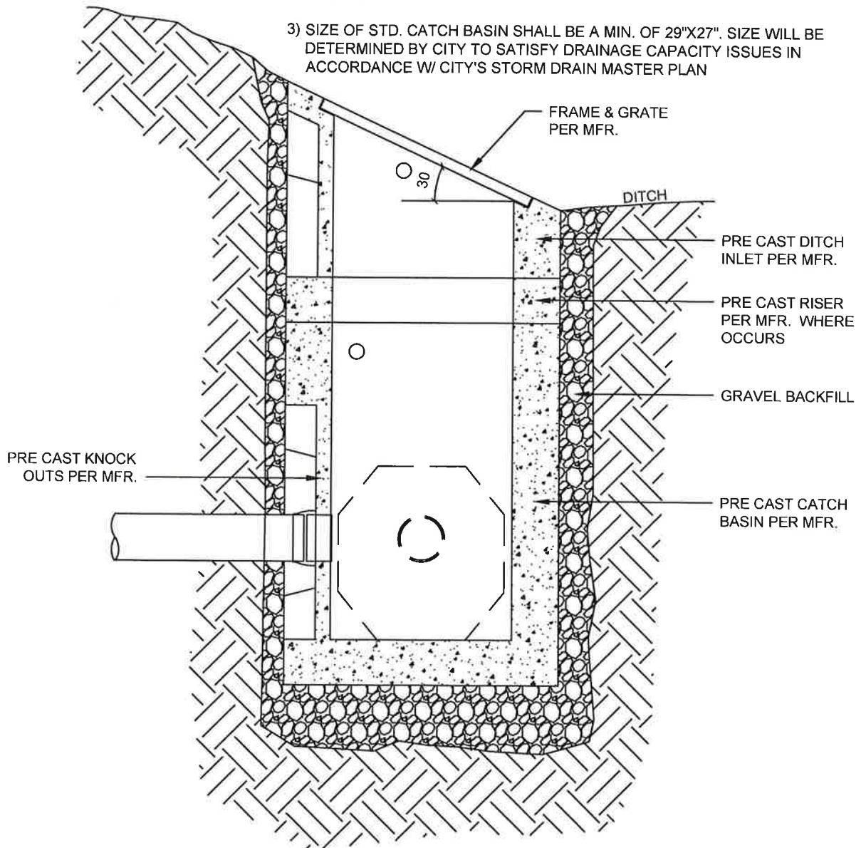
SECTION
