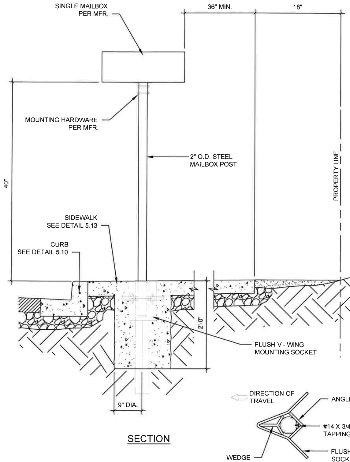
POST MOUNTING SOCKET
