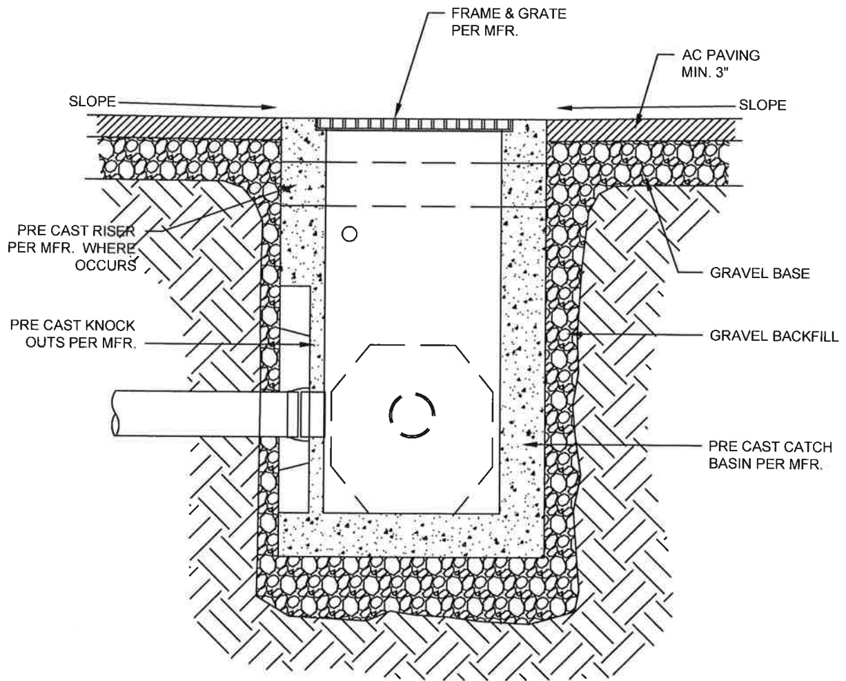
SECTION
