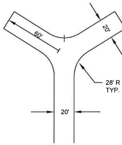
60' "Y"
