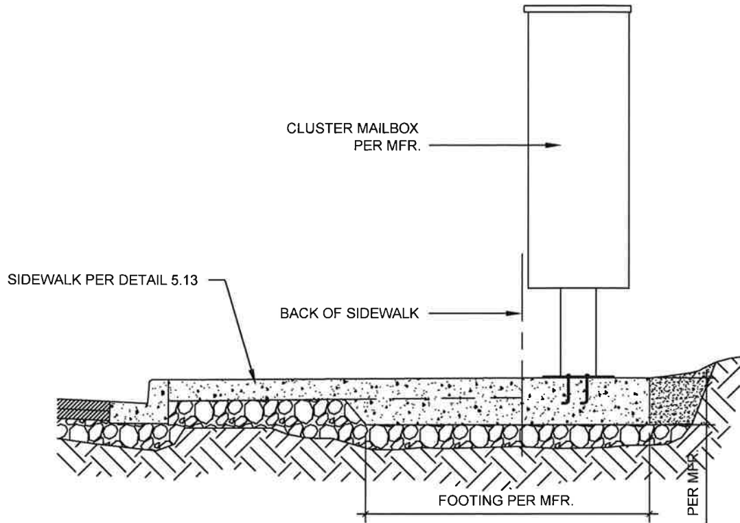
SECTION DETAIL
