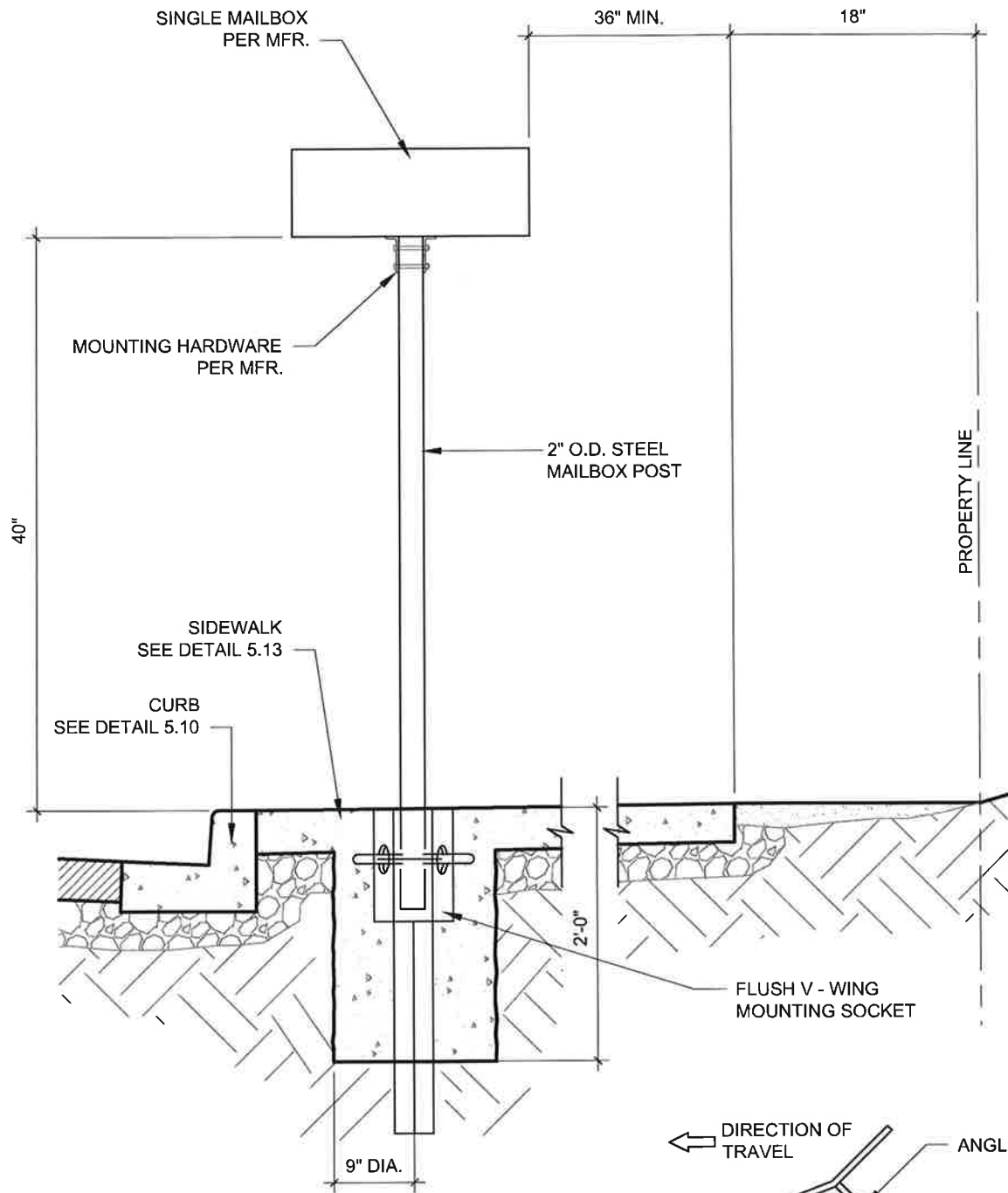
SECTION
